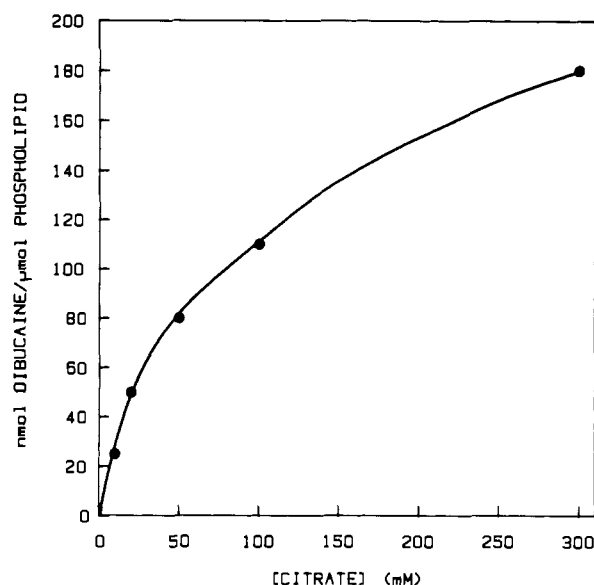
FIGURE 3: Effect of internal citrate concentration on the level of \Delta pH-dependent dibucaine uptake. Egg PC vesicles were prepared in the presence of the indicated citrate concentrations (pH 4.0), and subsequently, the exterior medium was exchanged for 20 mM Hepes/150 mM NaCl (pH 7.5). Vesicles (1 mM phospholipid) were incubated in the presence of 0.2 mM dibucaine. Uptake levels reflect values obtained after 1 h.
