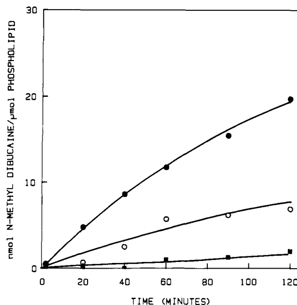
FIGURE 7: Uptake of N -methylidibucaine into LUVs at 22 °C. The LUVs (1 mM egg PC) were incubated in the presence of 0.2 mM N -methylidibucaine. The internal vesicle buffer was 169 mM K \text{Glu} /20 mM Hepes (pH 7.5). External buffers were (■) 169 mM K \text{Glu} /20 mM Hepes (pH 7.5) and (●, ○) 150 mM NaCl/20 mM Hepes (pH 7.5). Valinomycin was added (●, ■) to achieve 1 \mu\text{g}/\mu\text{mol} of egg PC.
