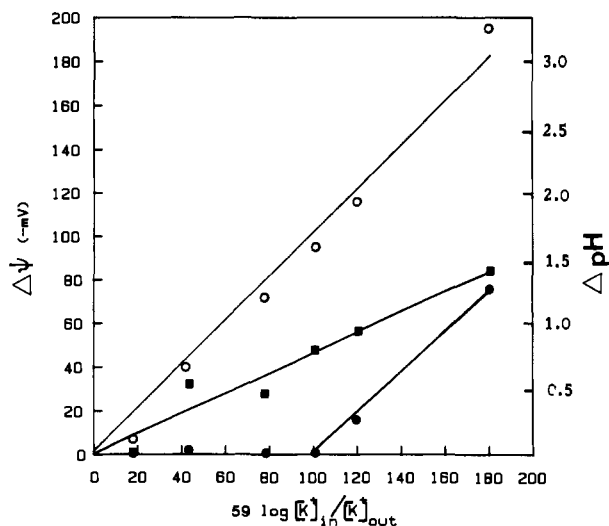
FIGURE 6: \Delta\psi (O) and \Delta\text{pH} (●, ■) as a function of the transmembrane \text{K}^+ gradient. Egg PC LUVs (1 mM lipid) having 169 mM K \text{Glu} /20 mM Hepes (pH 7.5) in the internal aqueous space were incubated in the presence of 1 \mu\text{g} of valinomycin/ \mu\text{mol} of egg PC. [ ^{14}\text{C} ]TPP (1 \mu\text{Ci}/\text{mL} ) or [ ^{14}\text{C} ]CH _3\text{NH}_2 (1 \mu\text{Ci}/\text{mL} ) was added to the samples for determination of \Delta\psi and \Delta\text{pH} , respectively. The indicated transmembrane \text{K}^+ gradients were achieved by passing the LUVs over Sephadex G-50 columns equilibrated with buffers consisting of 169 mM K \text{Glu} /20 mM Hepes (pH 7.5) and 150 mM NaCl/20 mM HEPES (pH 7.5) at ratios ranging from 50:50 to 0.1:99.9. Dibucaine was added (■) to achieve a final concentration of 0.1 mM.
